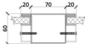
Middle Frame for glazed Partition
