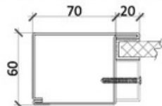
Side/top Frame for glaze Partition
